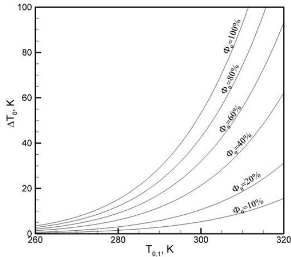
Figure 3: Total temperature increment on the condensation wave depending on total temperature at the inlet and on air relative humidity.
