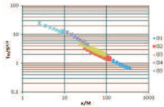
Figure 7: The decay power law (7b) behind grids.
