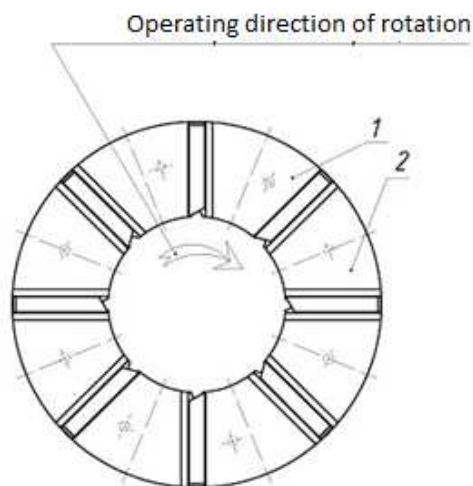
Figure 8: Thrust bearing with reversible and nonreversible pads: 1 – thrust nonreversible pad, 2 – thrust reversible pad.
