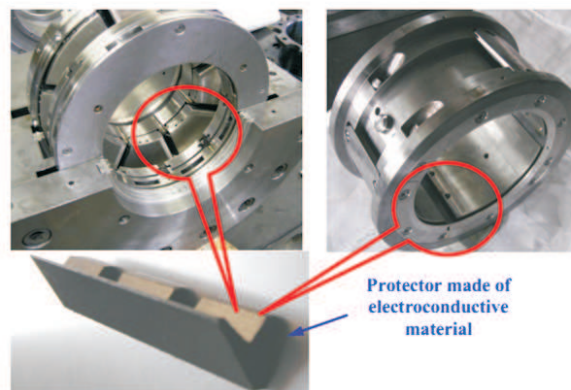
Figure 6: Bearings equipped with the scraper-protectors to prevent them from electroerosive deterioration.
