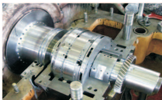
Figure 13: Journal-Thrust Bearing PDU –120/260 for Modernized Turbine 103JT.
