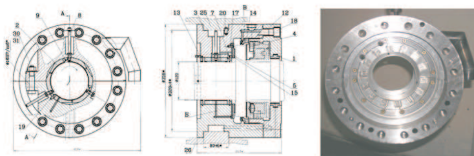
Figure 12: Journal-thrust bearing TRIZ.
