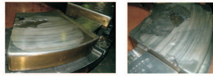
Figure 16: Destruction of the regular thrust pads.
