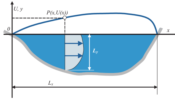
Figure 7: The mean velocity integration scheme in an irregular open channel cross section.
