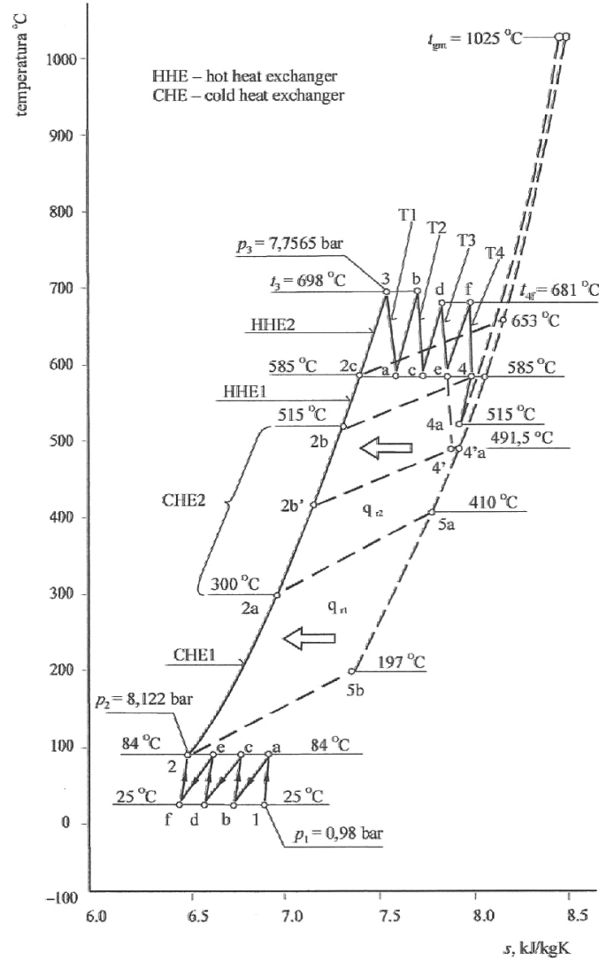
Figure 6. Temperature-specific entropy diagram for working air and exhaust for modified system with combustion in exhaust side: q_{R1} – heat supplied in exchanger CHE1, q_{R2} – in exchanger CHE2.
