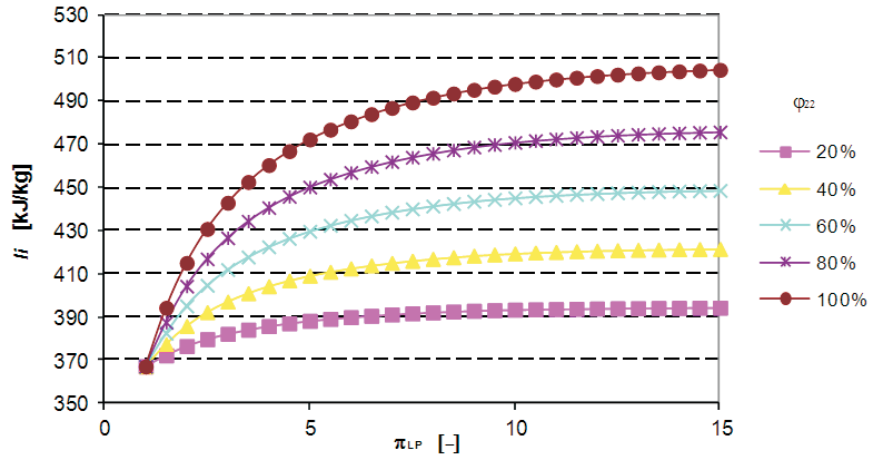
Figure 6. System internal unit work l_i versus compressor low-pressure part compression ratio \pi_{LP} and relative air humidity after humidification \phi_{22} .
