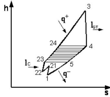
Figure 2. Thermodynamic cycle of gas system with heat regeneration and intercooling by water injection: q^+ , q^- – positive and negative heat (heat added, and removed), l_c , l_{GT} – internal work of compressor and turbine.
