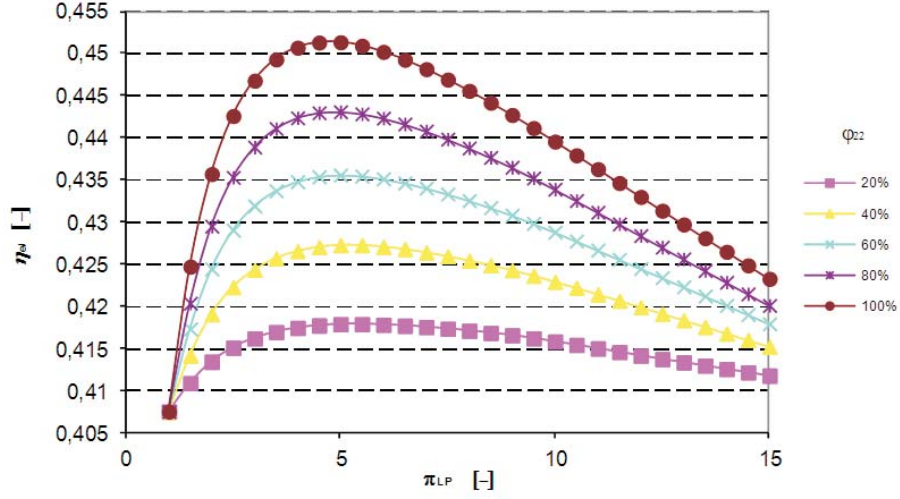
Figure 5. System electrical efficiency \eta_{el} versus compressor low-pressure part compression ratio \pi_{LP} and relative air humidity after humidification \phi_{22} .
