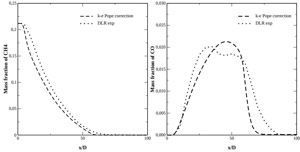
Figure 6. Mass fraction along centreline data, for \text{CH}_4 and \text{CO} .
