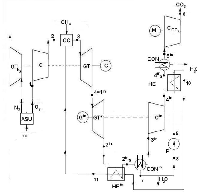
Figure 16. Schematic diagram of the double Brayton cycle with the use of oxy combustion, water injection and capture \text{CO}_2 (ASU – air separation unit, CC – combustion chamber, C – compressor, GT – gas turbine, HE – heat exchanger, G – electric generator, M – motor, CON – condenser, P – pump, \text{GT}_{\text{N}_2} – additional gas turbine of \text{N}_2 , \text{C}_{\text{CO}_2} – compressor of \text{CO}_2 ).
