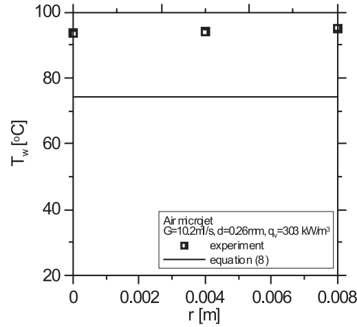
Figure 14. Wall temperature distribution on a plate after air microjet impingement, d = 260 \text{ } \mu\text{m} , \dot{m} = 10.2 \text{ ml/s} .
