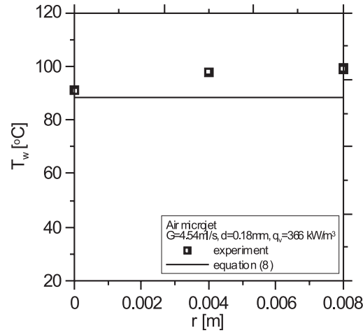
Figure 13. Wall temperature distribution on a plate after air microjet impingement, d = 180 \text{ } \mu\text{m} , \dot{m} = 4.54 \text{ ml/s} .
