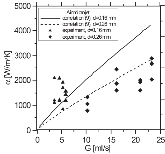
Figure 8. Fit to experimental data for two nozzle diameters, 180 and 260 \mu\text{m} to data for air.
