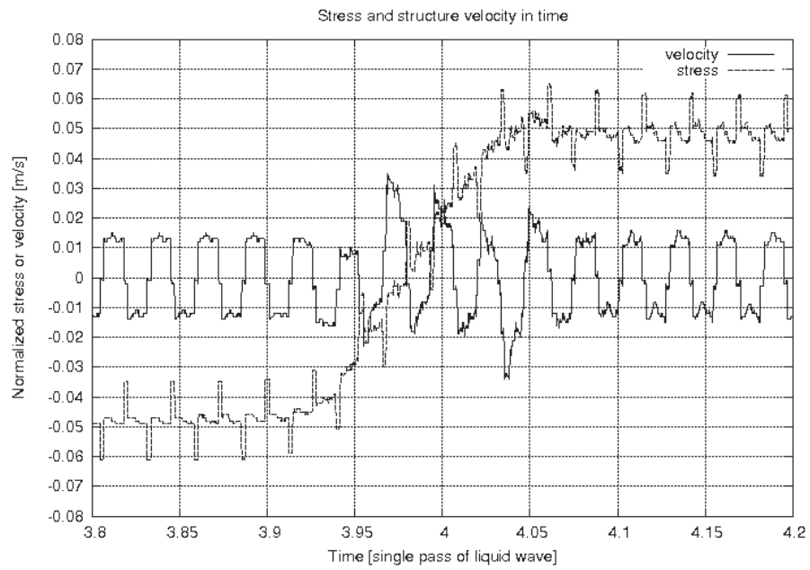
Figure 7. The stress and pipe wall velocity in time for the pipe with 48 inner supports.
