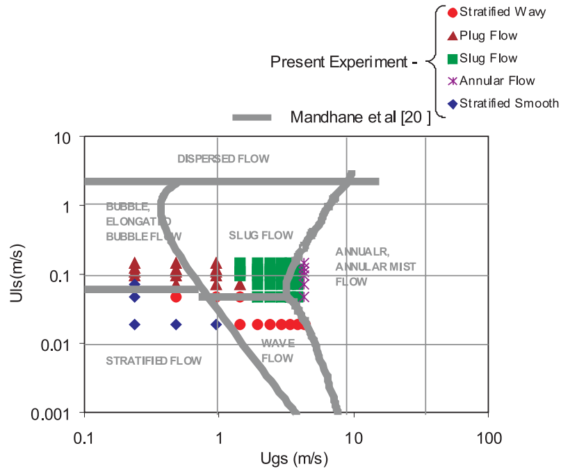
Figure 2. Two-phase flow regime map: comparison of the present results with the Mandhane et al. [20] flow map.
