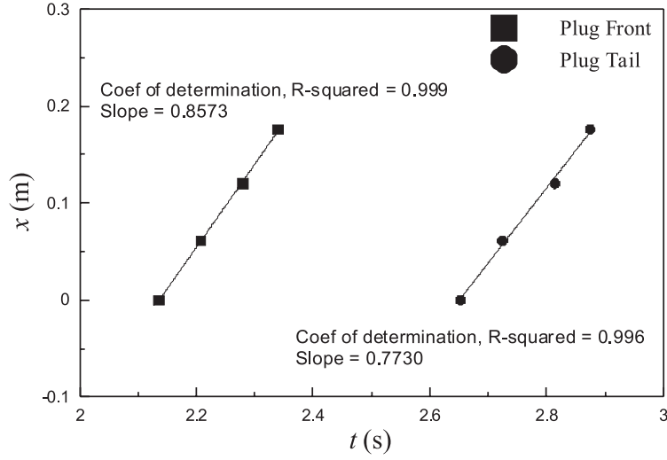
Figure 7. Plug front and tail trajectory for U_{ls} = 0.12 m/s and U_{gs} = 0.48 m/s.
