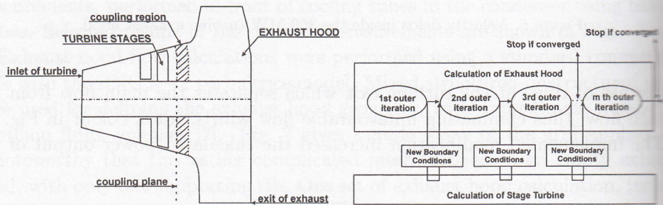
Figure 9. Coupled calculations of the turbine last stage/exhaust hood flow. Exhaust hood flow parameters are assumed in the coupling plane or in the overlapping area on the base of the turbine last stage calculations [13].
