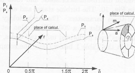
Figure 10. Radial and circumferential distributions of static and total pressure at turbine exit.
