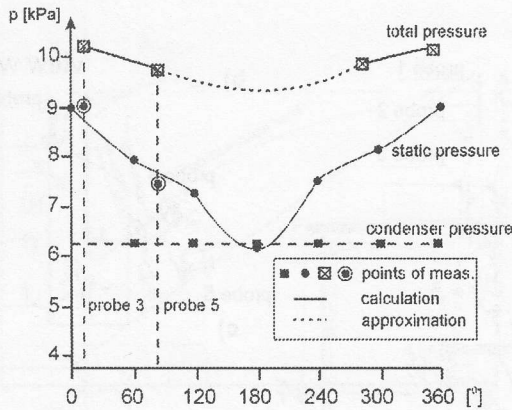
Figure 4. Circumferential distributions of static and total pressure at the last stage exit.
