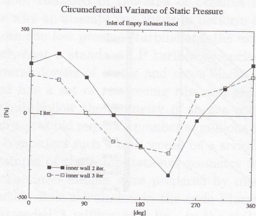
Figure 12. Comparison of circumferential static pressure distributions in iteration I, II and III (mid-span section).
