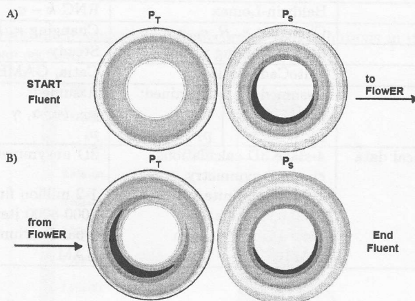
Figure 11. A) Uniform total pressure (left) and corresponding static pressure (right) distribution at diffuser inlet B) Total pressure (left) and corresponding static pressure (right) distribution at diffuser inlet (II iteration).
