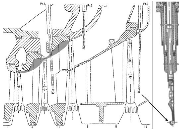
Figure 2. Thermal measurements equipment in the LP section of 200MW turbine with Bauman's stage; zones of influence of tip leakage flow are shadowed in grey
