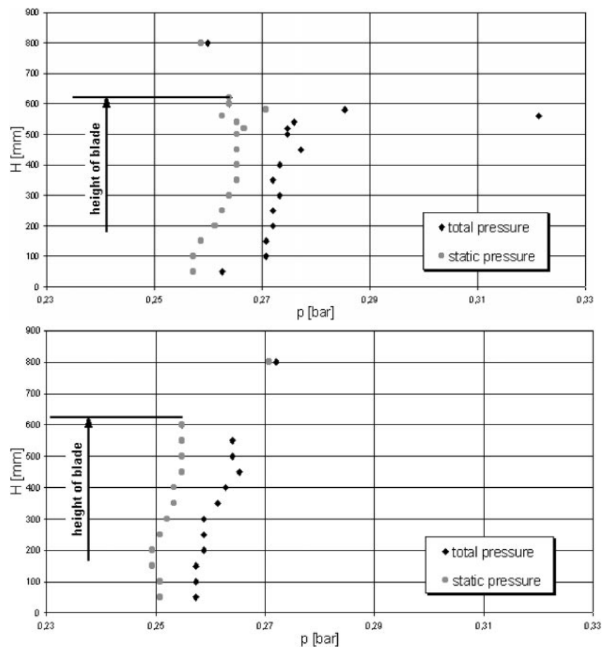
Figure 3. Distribution of total and static pressure along the height of probing before (upper diagram) and after (lower diagram) modernisation
