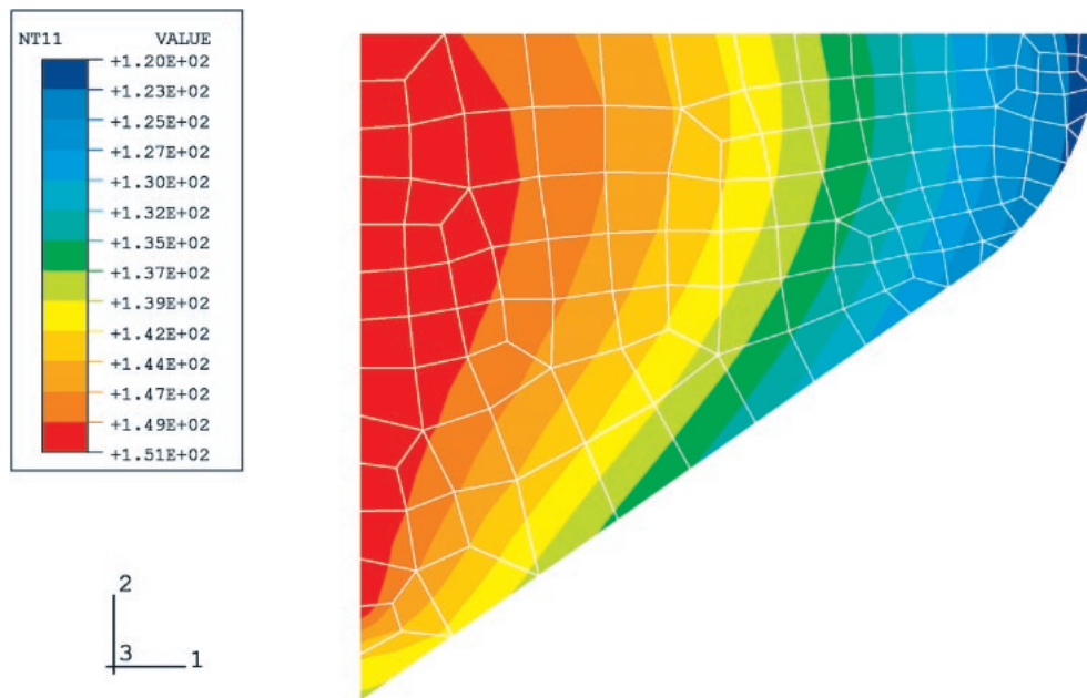
Figure 12. Calculated temperature distribution in casing at steam temperature 43°C (see Figure 11)
