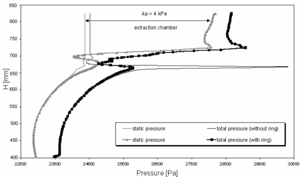
Figure 8. Comparison of computed pressure profile along the probing distance for the case with and without the ring
