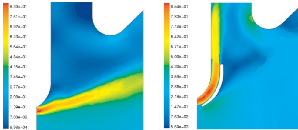
Figure 9. Distribution of Mach number before and after modernisation
