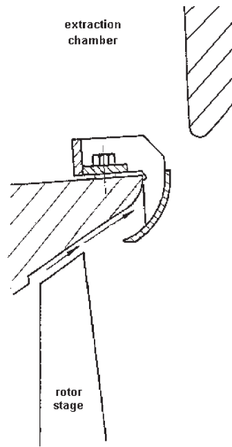
Figure 6. Proposal of ring installation under patent in the modernized exhaust
