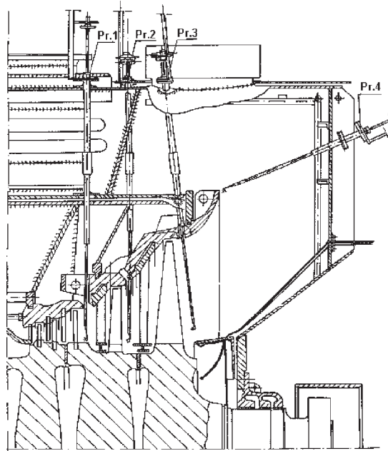
Figure 5. Measurement system in the new LP part of 200MW turbine
