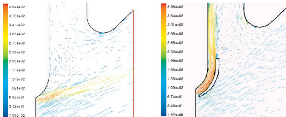
Figure 10. Velocity vectors before and after modernisation
