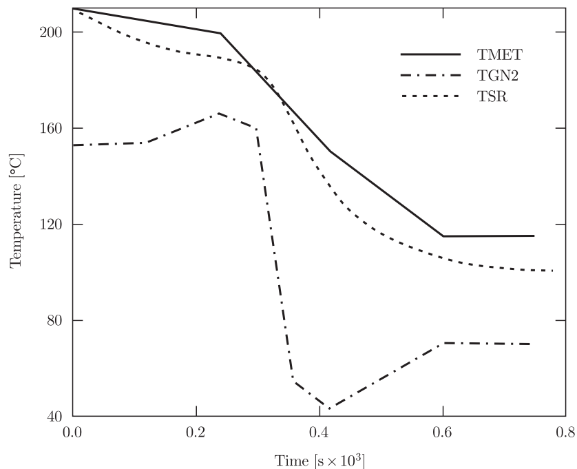
Figure 11. Temperature variation during warm start-up; TMET – casing temperature, TGN2 – measured steam temperature, TSR – calculated casing temperature in the region of clamping screws
