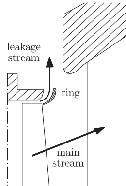
Figure 1. New design of the stage before extraction point
