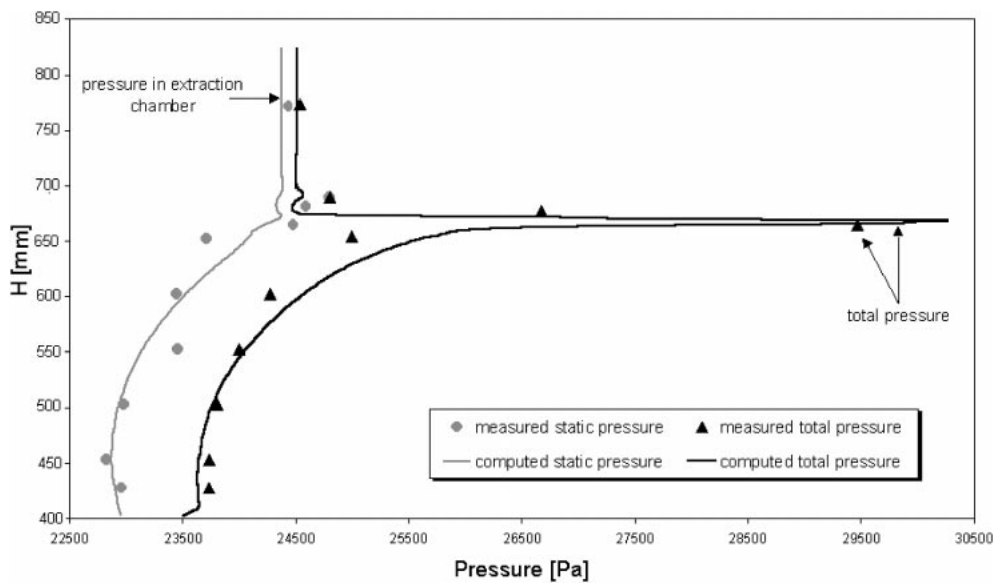
Figure 7. Comparison of computed and measured pressure profile along the probing distance for the case without the ring
