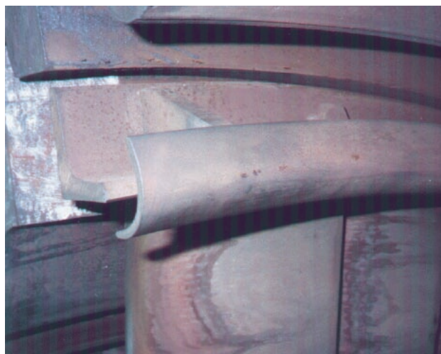
Figure 4. Ring inside the turbine flow path after six years of operation
