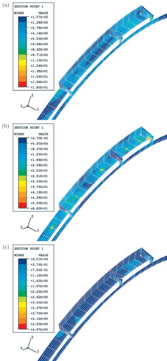
Figure 13. Huber-Mises reduced stresses [MPa] resulting from: (a) steady-state steam flow, (b) temperature difference during start-up, (c) unsteady steam load
