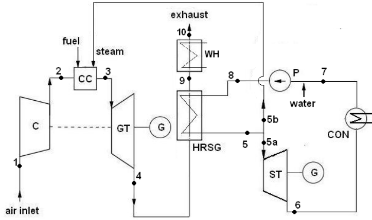
Figure 1. Scheme of the gas-steam power unit with the possible utilisation of steam in the Cheng cycle: GT – gas turbine, C – compressor, CC – combustion chamber, G – electric generator, HRSG – heat recovery steam generator, ST – steam turbine, P – pump, CON – condenser, WH – water heater.
