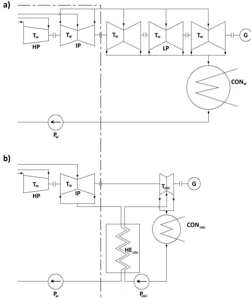
Figure 1: Schematic of the concept of the Szewalski binary vapour cycle b) comparison to conventional steam cycle a). LP – low-, IP –intermediate-, HP – high-pressure part of steam turbine, respectively, HE_{ORC} – regenerative heat exchangers, P_w – pump of water, G – generator, CON_w – condenser of water steam, T_w – turbine of steam, T_{ORC} – turbine of low boiling point fluid, P_{ORC} – pump of low boiling point fluid, CON_{ORC} – condenser of vapour of low boiling point fluid [23].
