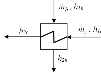
Figure 6: Schematic of steam cooler and regenerative heat exchangers.
