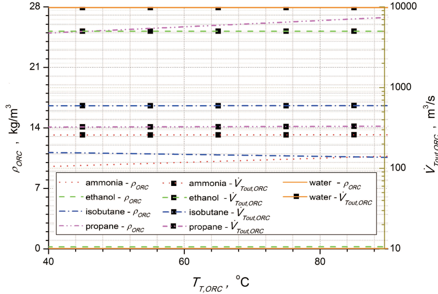
Figure 11: Density of vapour at the outlet of ORC turbine, \rho_{ORC} , and volume flow rate at the outlet of ORC turbine, \dot{V}_{Tout,ORC} , vs. temperature of vapour before turbine, T_{T,ORC} , and the type of low boiling point fluid.
