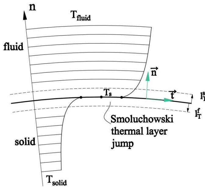
Figure 1. Temperature profile in a solid-fluid contact layer
