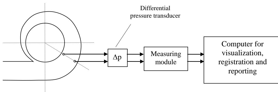
Fig. 1. Block diagram of continuous measurement of flow rate through the turbine by means of the differential pressure method
