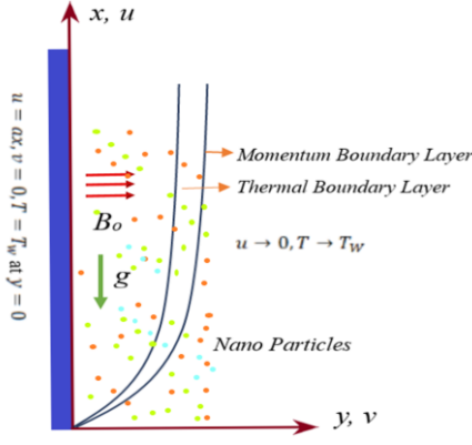
Fig. 1. Schematic flow diagram.
