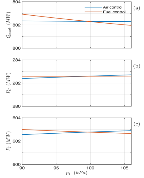
Fig. 9. Influence of the air pressure p_1 at the compressor inlet on: (a) heat flux supplied in the combustion chamber \dot{Q}_{comb} , (b) internal power of the compressor P_C , (c) internal power of the turbine P_T .
