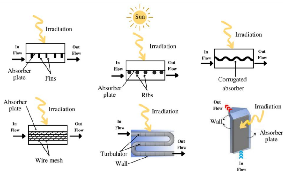
Fig. 1. Modifications implemented in solar air heaters.
