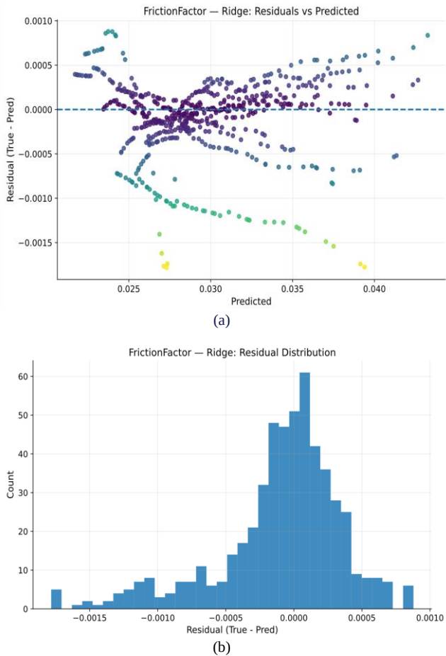
Fig. 17. OOF residual diagnostics for friction factor – ridge regression: (a) residual vs. predicted and (b) residual distribution.
