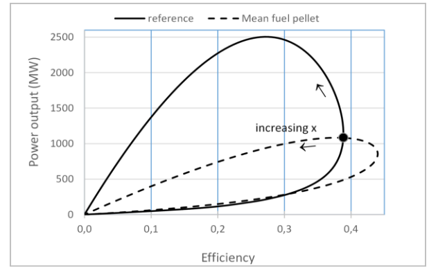
Fig. 8: Power output as a function of efficiency ( \alpha = 1000 W/(K m 2 )).
