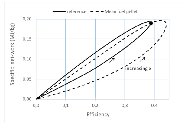
Fig. 9: Cycle net work as a function of efficiency ( \alpha = 1000 W/(K m 2 )).
