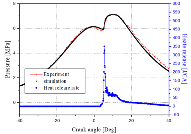
Fig. 5. The cylinder pressure (experimental vs. calculated) and heat release rate evolution.
