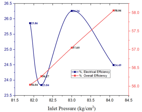
Fig. 3. Electrical efficiency and overall efficiency vs. inlet pressure at 507°C.
