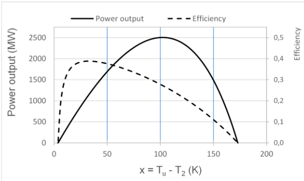
Fig. 7: Power output and efficiency as a function of x = T_u - T_2 (reference PWR case and \alpha = 1000 W/(K m 2 )).
