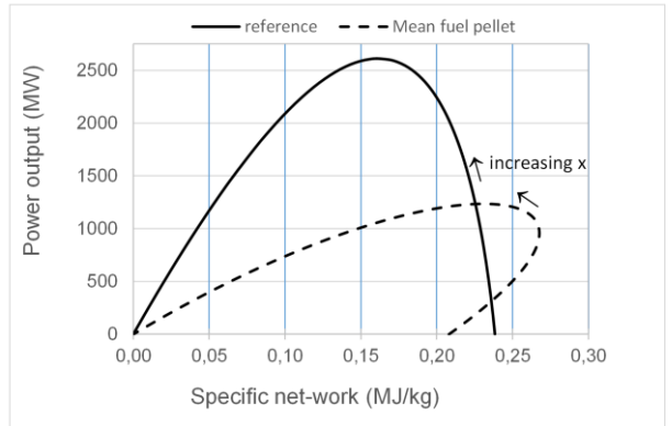
Fig. 5. Power output as a function of the specific net work for x = T_u - T_2 variation.
