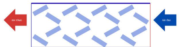
Fig. 59. Roughness element in the form of novel staggered cuboid baffles (drawn after [140]).
